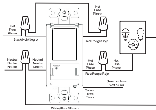
Unipolaire, 125VAC
